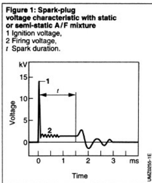
typical spark
